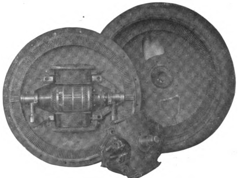
WHEEL DISSEMBLED, SHOWING MOTOR FIELDS AND ARMATURE.
